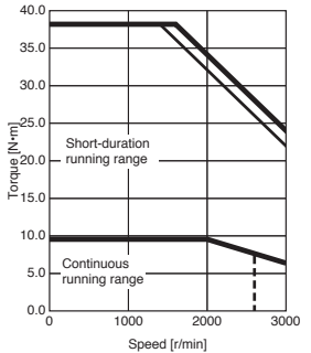
HK-KT2024W Torque increased
