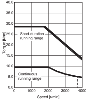
HK-ST2024W Standard torque
