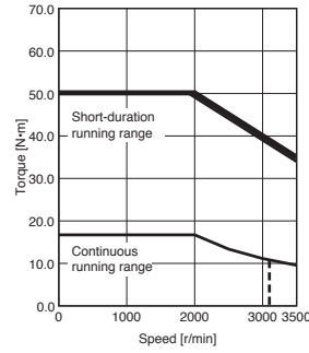
HK-ST3524W Standard torque
