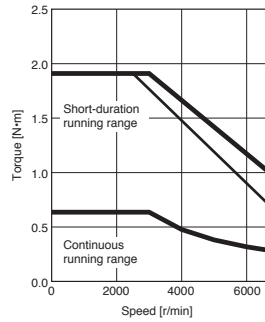
HK-MT23W Standard torque
