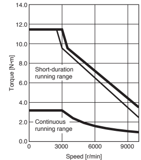
HK-MT103VW Torque increased
