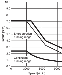
HK-MT7M3VW Standard torque
