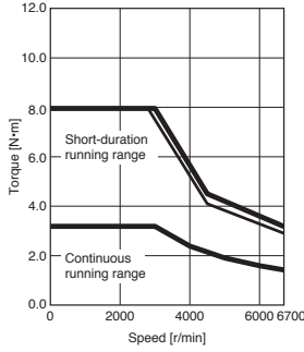
HK-RT1034W Standard torque
