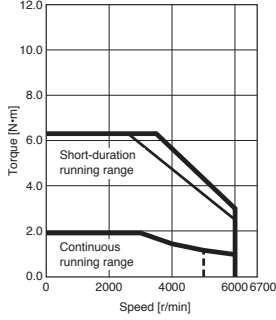
HK-KT63UW Standard torque
