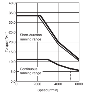
HK-RT3534W Torque increased
