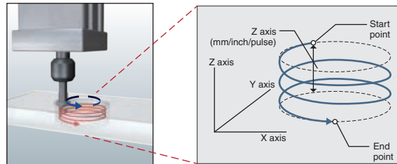
Helical interpolation
