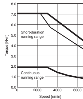
HK-MT63W Torque increased
