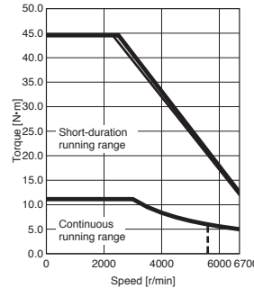
HK-ST3534W Torque increased
