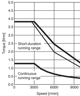
HK-MT43VW Standard torque
