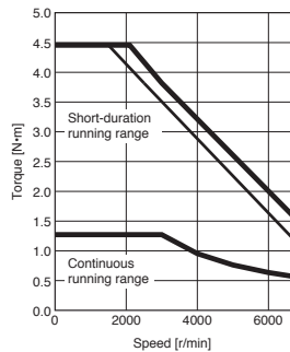
HK-MT43W Torque increased
