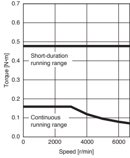
HK-MT053W Standard torque
