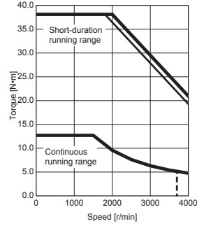
HK-ST2024W Torque increased
