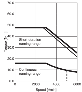
HK-ST5034W Standard torque
