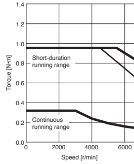
HK-MT13W Standard torque
