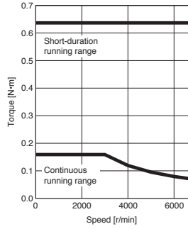
HK-MT053W Torque increased
