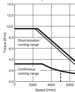
HK-MT103W Standard torque
