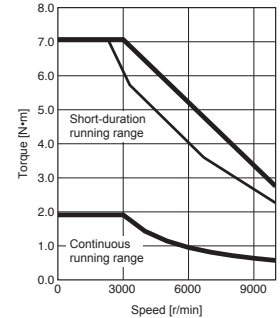
HK-MT63VW Torque increased
