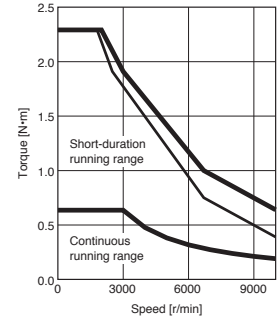
HK-MT23VW Torque increased
