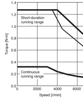
HK-MT13W Torque increased
