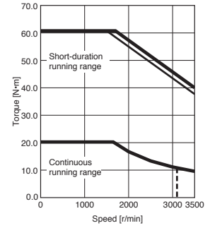
HK-ST3524W Torque increased
