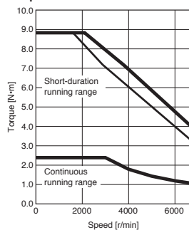
HK-MT7M3W Torque increased
