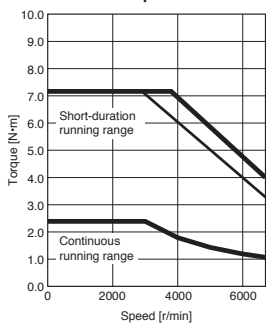
HK-MT7M3W Standard torque
