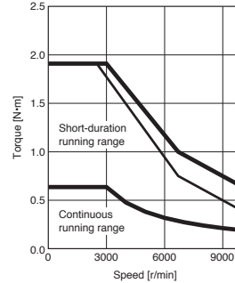
HK-MT23VW Standard torque
