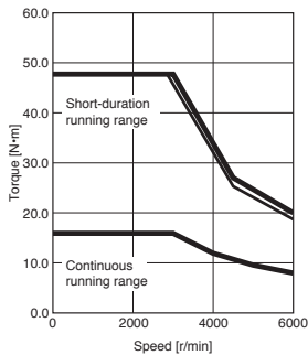
HK-RT5034W Standard torque
