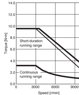
HK-MT103VW Standard torque
