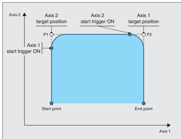
Triggered motion
