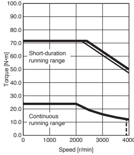
HK-ST5024W Standard torque
