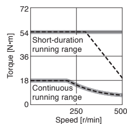
TM-RFM072G20 (Note 1, 3)
