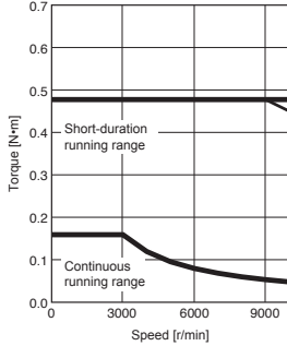
HK-MT053VW Standard torque
