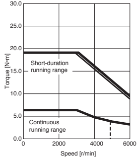
HK-KT2034W Standard torque
