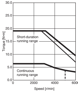
HK-KT203W Standard torque
