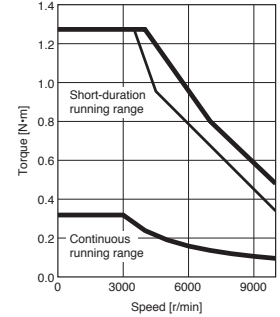
HK-MT13VW Torque increased
