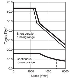
HK-ST5034W Torque increased
