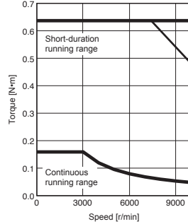
HK-MT053VW Torque increased
