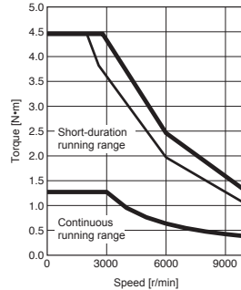
HK-MT43VW Torque increased
