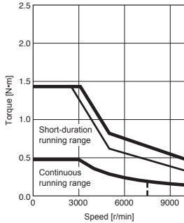
HK-MT1M3VW Standard torque
