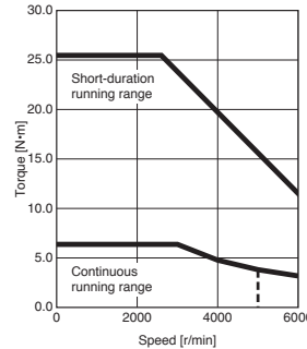
HK-KT203W Torque increased
