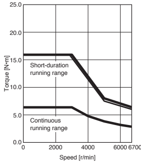
HK-RT2034W Standard torque
