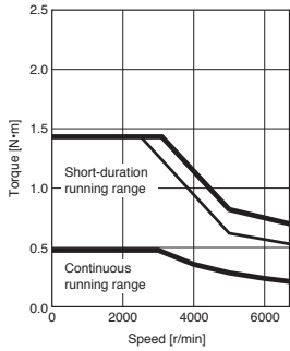
HK-MT1M3W Standard torque
