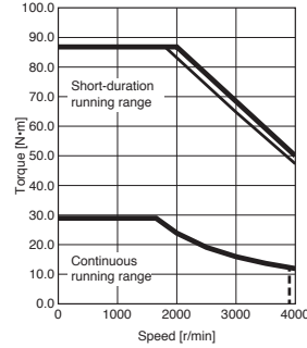
HK-ST5024W Torque increased
