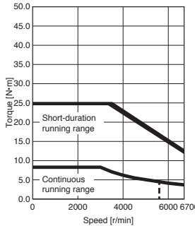
HK-ST3534W Standard torque
