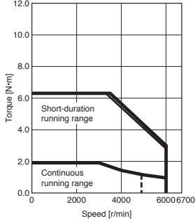
HK-KT634UW Standard torque
