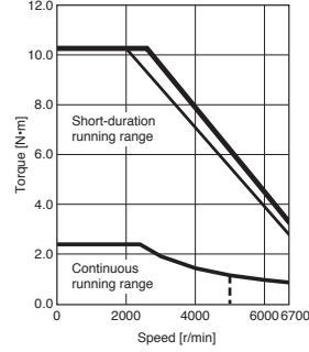
HK-KT63UW Torque increased
