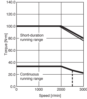
HK-ST7024W Standard torque
