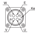
Encoder connector Servo motor flange direction → Electromagnetic brake connector Servo motor flange direction → Power connector Servo motor flange direction →
