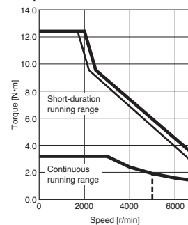
HK-MT103W Torque increased
