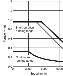
HK-MT13VW Standard torque
