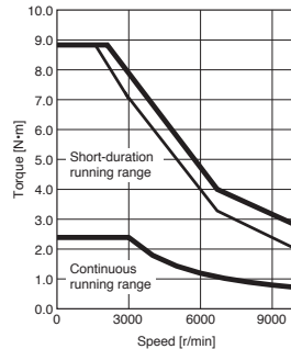
HK-MT7M3VW Torque increased
