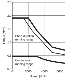
HK-MT1M3W Torque increased
