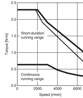
HK-MT23W Torque increased
