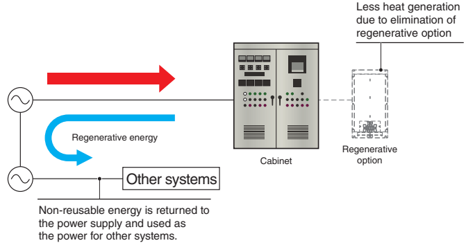
[Power regeneration system]
