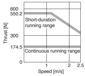
LM-AJP4D-45N-JSS0 (Note 1, 2, 3)
