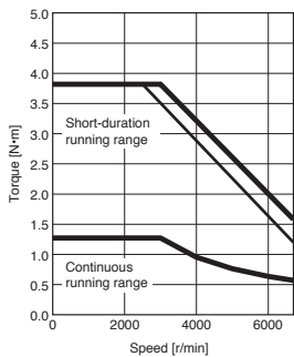
HK-MT43W Standard torque
