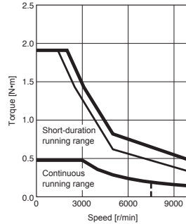
HK-MT1M3VW Torque increased
