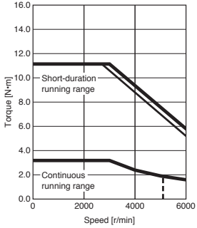
HK-KT103UW Standard torque
