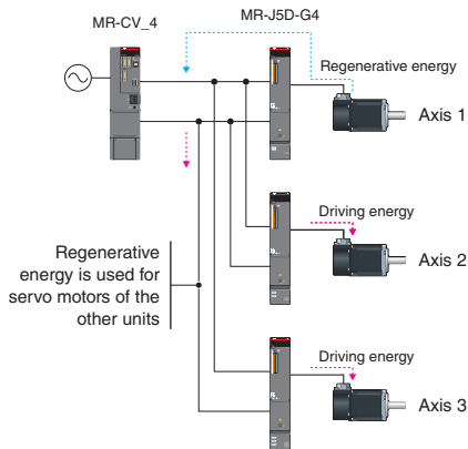
[Common DC bus connection]
