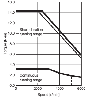
HK-KT103UW Torque increased
