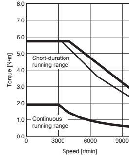
HK-MT63VW Standard torque
