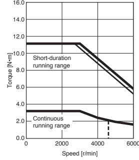
HK-KT1034UW Standard torque
