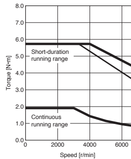
HK-MT63W Standard torque
